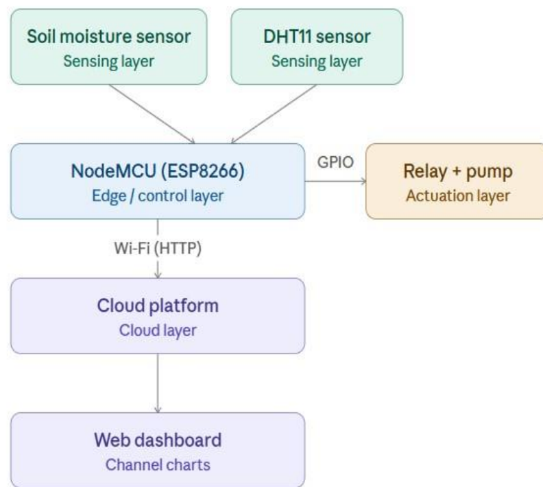
Fig. 1 Layered IoT system architecture
