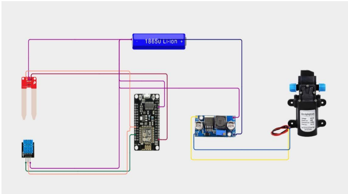
Fig. 2 Circuit wiring diagram
